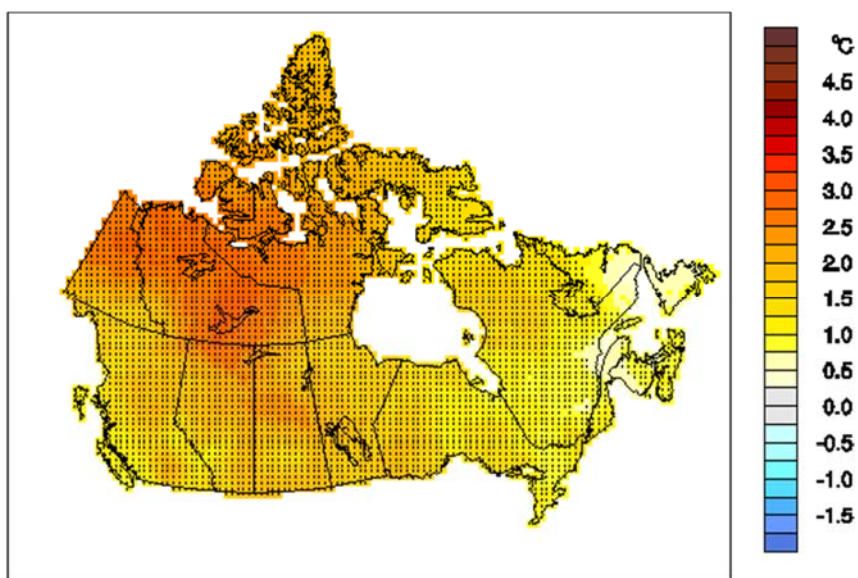
Trends in annual mean temperature for 1948-2012 (°C for 65 years). Grid squares with trends statistically significant at the 5% level are marked with a dot.
